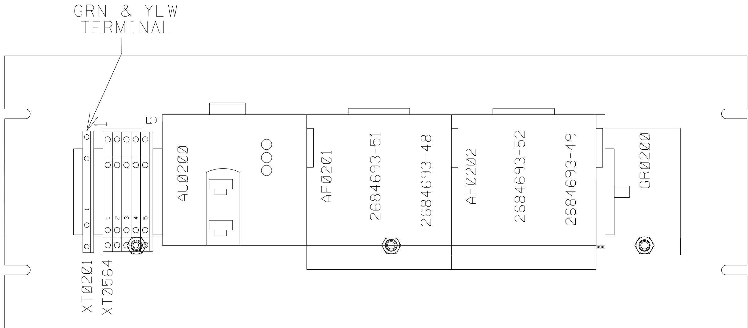
BACK VIEW WITH FLEX I/O INSTALLED TYP. FOR XT0564
